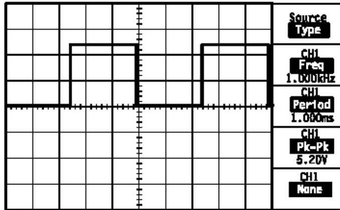
Figure 9. Measure Function Menu
