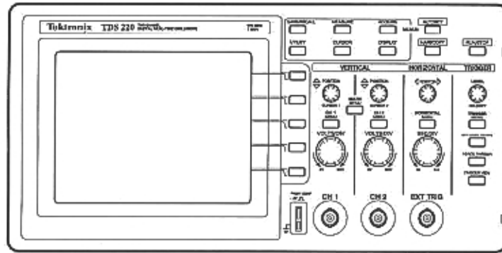
Figure 4. Front Panel of the Oscilloscope
