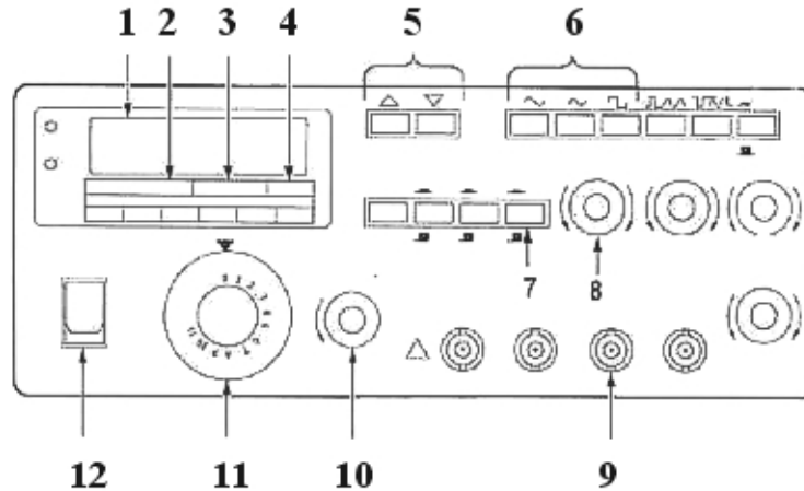
Figure 3. Front Panel of the Function Generator
