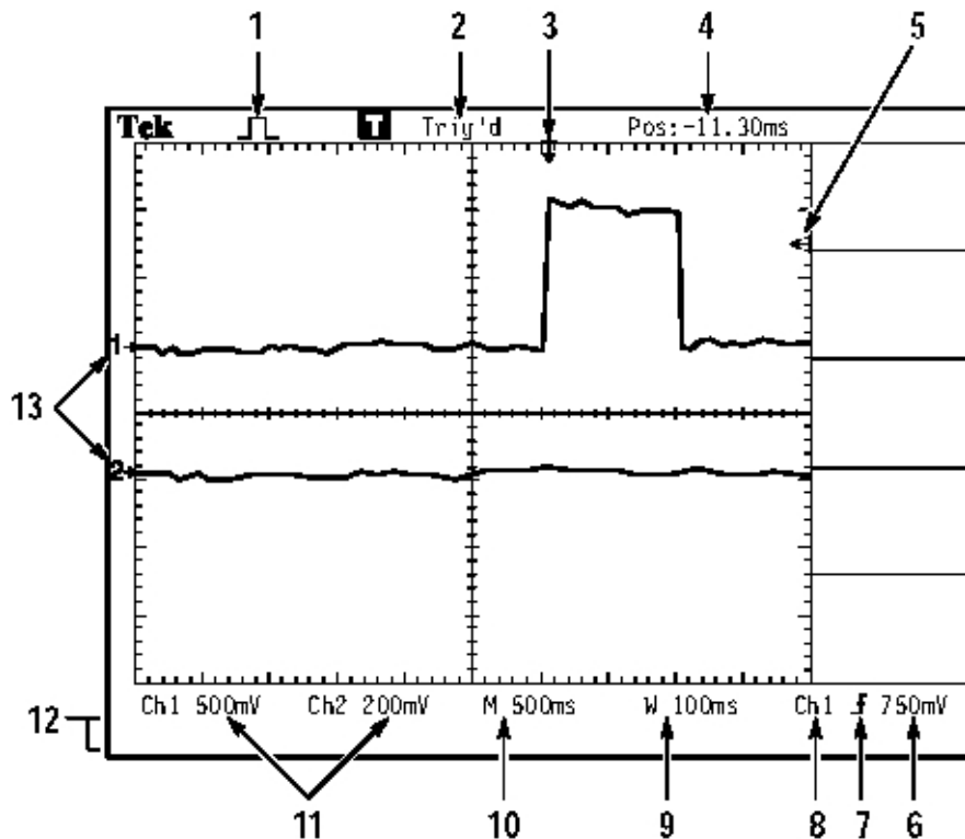
Figure 5. Oscilloscope Display
