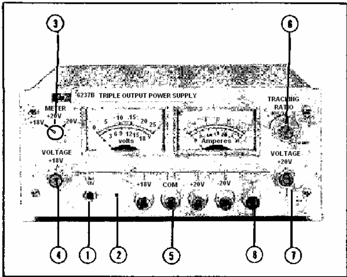
Figure 2. Front Panel of the HP6237B DC Power Supply
