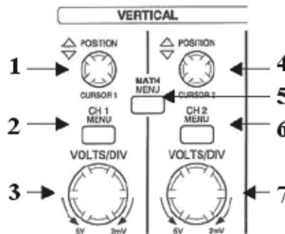
Figure 6. Vertical Controls
