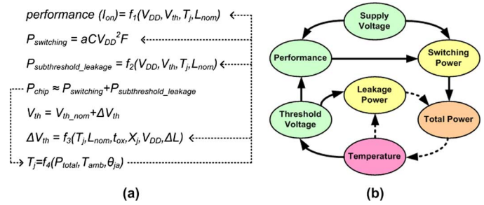
Fig. 8. (a) Models for various metrics are expressed in functional format. Couplings are indicated using broken lines. T_j represents the operating temperature, L_{\text{nom}} is the nominal gate length, a is the switching activity, C is the total load capacitance, F is the operating frequency, V_{\text{th\_nom}} denotes the nominal threshold voltage, \Delta V_{\text{th}} is the change of threshold voltage, t_{\text{ox}} is the gate oxide thickness, X_j is the junction depth, \Delta L is the change of gate length due to variation, T_{\text{amb}} denotes the ambient temperature, and \theta_{ja} denotes the equivalent junction-to-ambient thermal resistance. (b) Schematic view of electrothermal couplings between different design parameters. As technology scales, the couplings between power, leakage, and temperature (shown by dotted arrows) become increasingly prominent.
