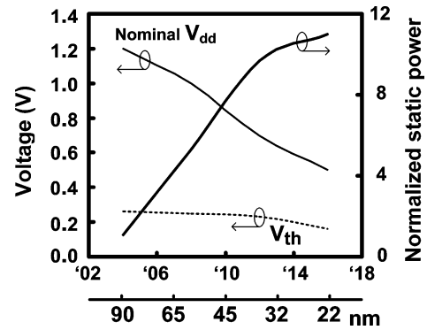
Fig. 5. Trends of nominal supply voltage, threshold voltage, and normalized static power based on ITRS [2].
