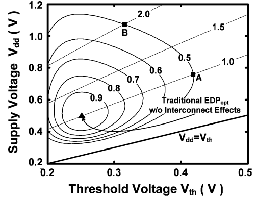
Fig. 2. Traditional $V_{dd}/V_{th}$ optimization uses EDP as a design metric (without considering the effect of interconnects). The EDP contours and iso-performance curves are obtained by simple numerical calculation without considering electrothermal couplings between temperature and static power dissipation at 100-nm technology node. Note that although five EDP contours (0.9, 0.8, 0.7, 0.6, 0.5) and three iso-performance curves (1.0, 1.5, 2.0) are drawn in this figure, other values of EDP contour and iso-performance curve can be easily employed.
