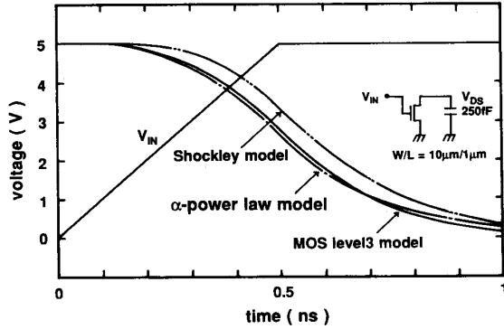
Fig. 6. Comparison of discharging waveforms calculated with the Shockley model, the present model, and SPICE MOS level 3 model.
