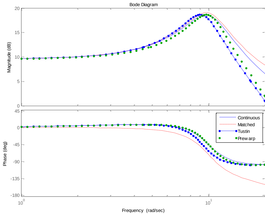
Figure 1: Bode Plot of Various Systems in Problem 5
