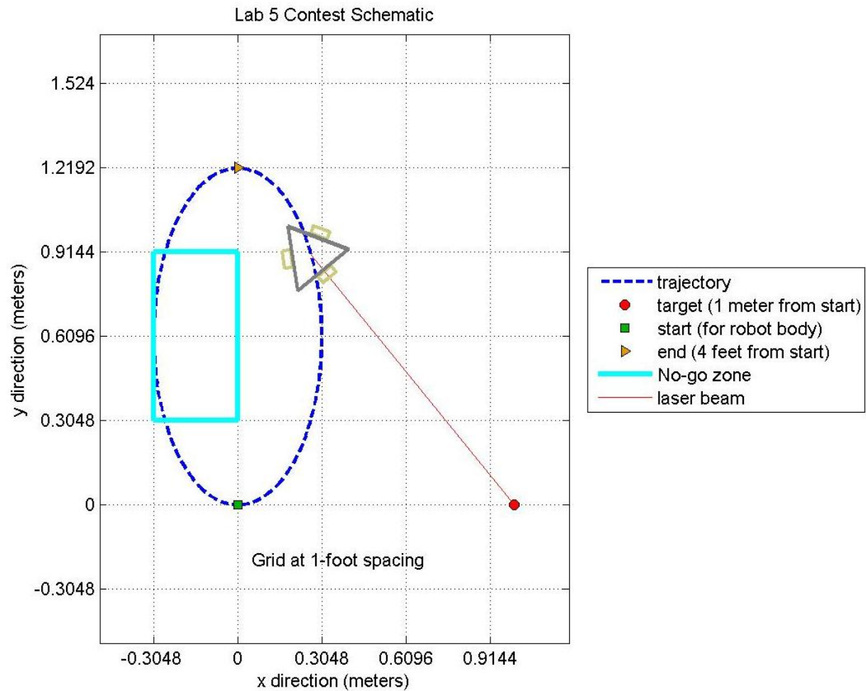
Figure 1. Schematic for the Omnibot Contest. Each team must design a controller that will move the omnibot from “start” to “end” while simultaneously pointing a laser at the “target” and avoiding the “no-go zone”.
