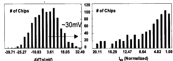
Figure 2: Die-to-die V_t , I_{sb} variation
