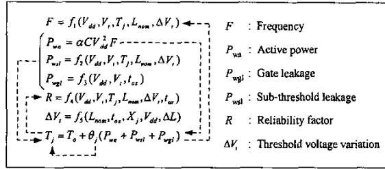
Fig.5. Models for various metrics are expressed in functional format. Electrothermal couplings are indicated using broken lines.
