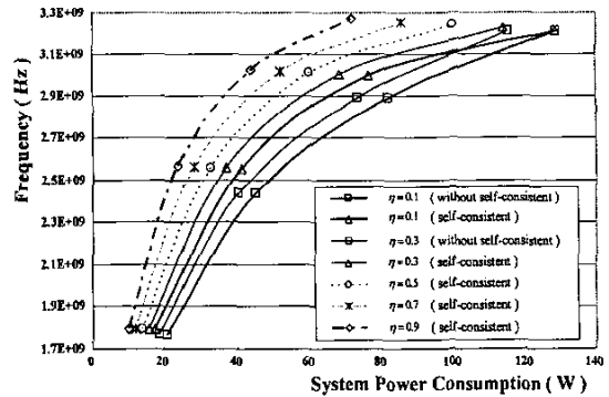
Fig.12b. Frequency vs. system power consumption at different cooling efficiency ( \eta ). The junction-to-ambient thermal impedance, \theta_{ja} = 0.85 . For \eta = 0.1 and 0.3, the non self-consistent frequency is also plotted showing the advantage of employing the self-consistent method.
