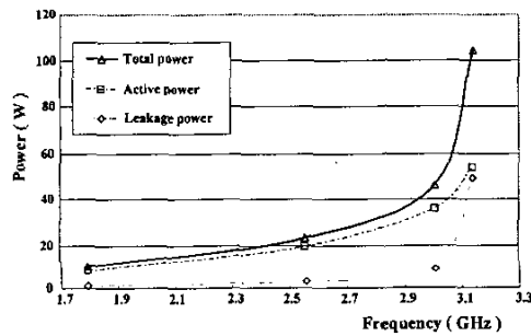
Fig.10. Self-consistent power consumption as a function of frequency using a) I_{on}/I_{off}=660 and b) I_{on}/I_{off}=220 .
