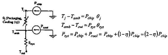
Fig.6. An equivalent thermal circuit illustrating relationship between junction , ambient , and external temperatures in terms of chip and system level power dissipation and thermal impedances. Typically, T_{amb} \approx 45^\circ\text{C} , T_{out} \approx 25^\circ\text{C} . The value of \theta_{sys} was estimated to be 0.285^\circ\text{C/W} for the IC.
