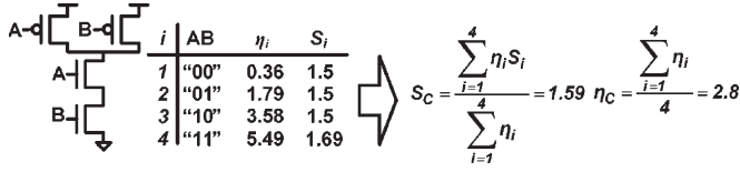
Fig. 17. Estimation of the average nominal value and spread for a NAND gate using (42).
