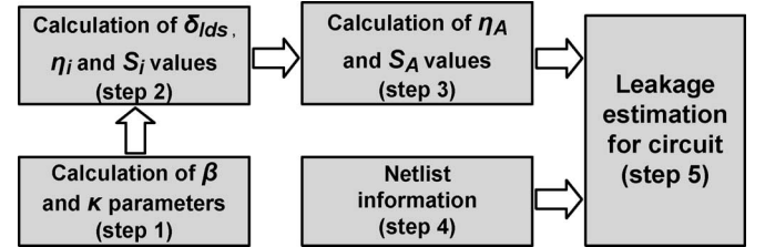
Fig. 19. Block diagram of leakage estimation of complex circuits using the proposed methodology.
