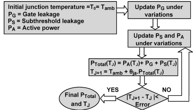
Fig. 11. Self-consistent evaluation of junction temperature and power dissipation under P–V–T variations [22]. Error is defined as a fraction of junction temperature ( T_j ); for example, algorithm can be executed until |T_{j+1} - T_j| < 0.01T_j .
