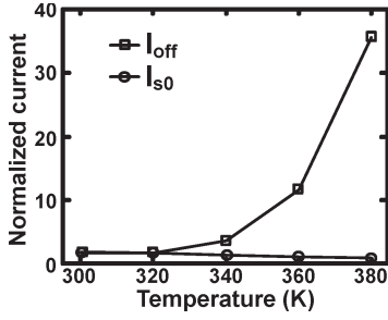
Fig. 6. Temperature dependence of I_{OFF} and I_{S0} .
