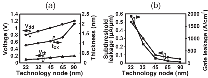
Fig. 2. (a) Supply voltage ( V_{dd} ), threshold voltage ( V_{th} ), and oxide thickness ( t_{ox} ) scaling predicted by the ITRS [3]. (b) Subthreshold and gate leakages predicted by the ITRS for NMOS devices at different technology nodes [3].
