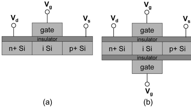
Fig. 1. Simulated Tunnel n-FETs. (a) Single-gate. (b) DG. SiO 2 and high- \kappa gate dielectrics were studied. t_{\text{dielectric}} = 3 nm (physical) and L_{\text{intrinsic}} = 50 nm. Drain doping ( n+ ) = 5 \times 10^{18} atoms/cm 3 and source doping ( p+ ) = 10^{20} atoms/cm 3 .
