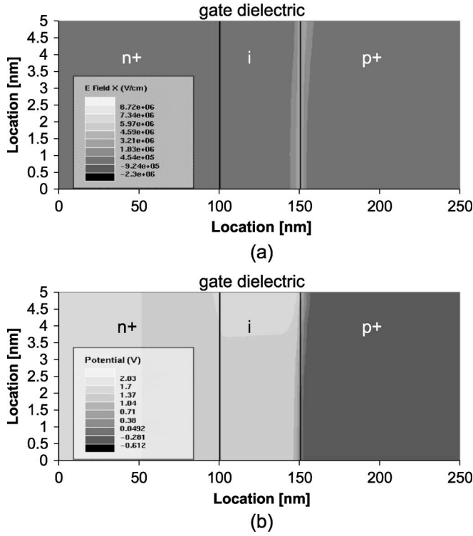
Fig. 14. (a) Contour plot of the x -component of the electric field in a single-gate Tunnel FET biased with V_d = 1 V and V_g = 1.8 V, in overdrive, with t_{\text{dielectric}} = 3 nm and \epsilon_{\text{dielectric}} = 29 . (b) Contour plot of the potential of the same device under the same bias conditions.
