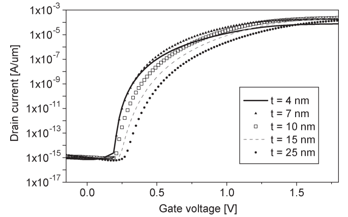
Fig. 9. DG-Tunnel-FET I_d - V_g characteristics for various silicon body thicknesses. L_{\text{intrinsic}} = 50 nm, t_{\text{dielectric}} = 3 nm, and \epsilon_{\text{dielectric}} = 29 . V_d = 1 V.
