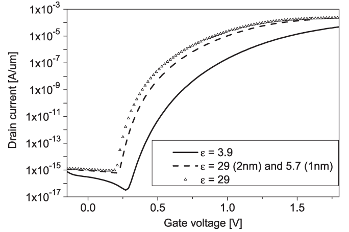
Fig. 8. DG-Tunnel-FET characteristics for a structure with 2 nm of a high- \kappa dielectric ( \epsilon_{\text{dielectric}} = 29 ) with a 1-nm interfacial layer of oxynitride ( \epsilon_{\text{dielectric}} = 5.7 ), compared with structures having 3 nm of the high- \kappa dielectric or 3 nm of SiO 2 . V_d = 1 V.
