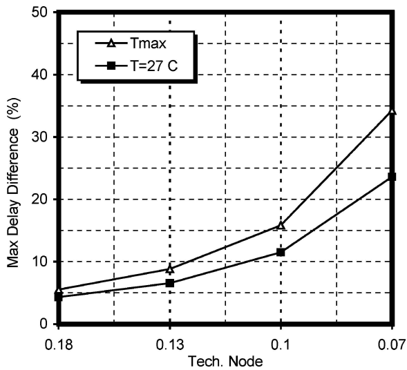
Fig. 11. Maximum percentage of the delay difference among drivers in a clock tree connected to a local power trunk for different technologies at room temperature, and at maximum interconnect temperature.
