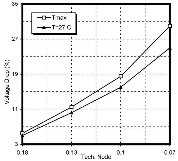
Fig. 5. Worst-case percentage of voltage-drop increase as a function of technology node for combined global/semi-global power grids considering the effects of self-heating, while allocating 10% of the routing area to the power network and assuming uniformly distributed on-chip decoupling capacitors.
