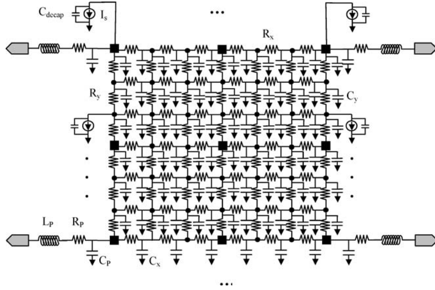
Fig. 1. RC model of a top-level global/semi-global power grid distribution network. Each intermediate node is connected to underlying circuit blocks modeled as time-varying current sources, I_s 's, and on-chip decoupling capacitances C_{decap} 's. The square nodes are the power pad pins connected by to the package pins through the RLC model of the package ( R_p , L_p , C_p ). Assuming a ball grid type of pin assignments in the package, the power pads are uniformly distributed over the chip area in our problem setup.
