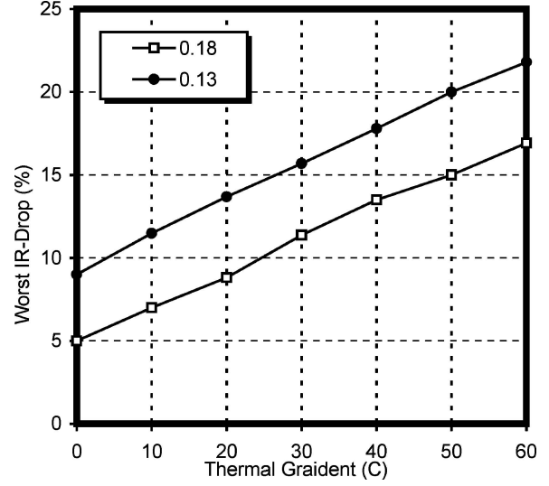
Fig. 9. Worst-case voltage-drop ( V_{\text{IR}}/V_{\text{dd}} ) increase (based on Fig. 5) in the presence of hot spots modeled by constant-peak Gaussian distribution as a function of thermal gradient magnitudes ( ^{\circ}\text{C} ), shown for two different technology feature sizes.
