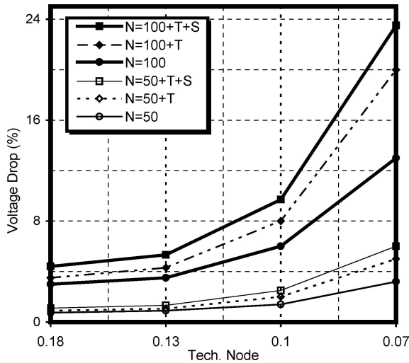
Fig. 7. Worst-case percentage of voltage-drop increase as a function of technology node in the presence of maximum interconnect temperature ( T ) and surface scattering/barrier effects ( S ), in the local power trunk lines. Notice that in this graph ( V_{dd} - V_{dd'} ) is the actual voltage over the two sides of the local power trunks, and N is the number of standard cells connected to the power trunk.
