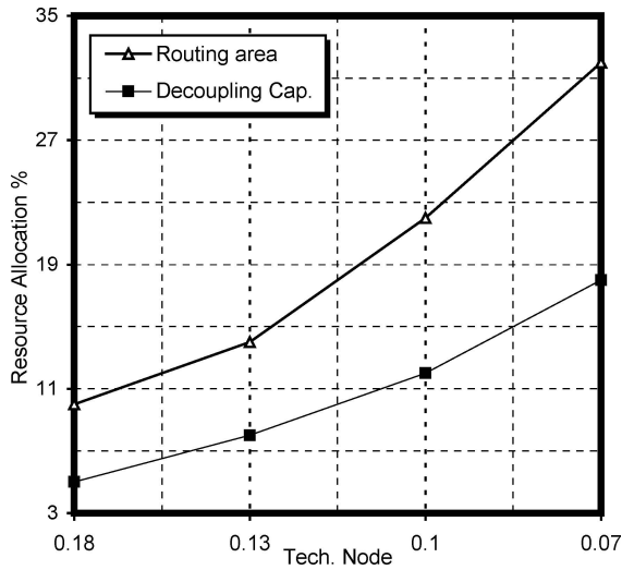
Fig. 6. Minimum required percentage of the allocated resources (global layer routing area for wire sizing and substrate area for decoupling capacitances) to ensure a worst-case 10% voltage drop for future technologies, considering the maximum temperature of global/semi-global interconnects.
