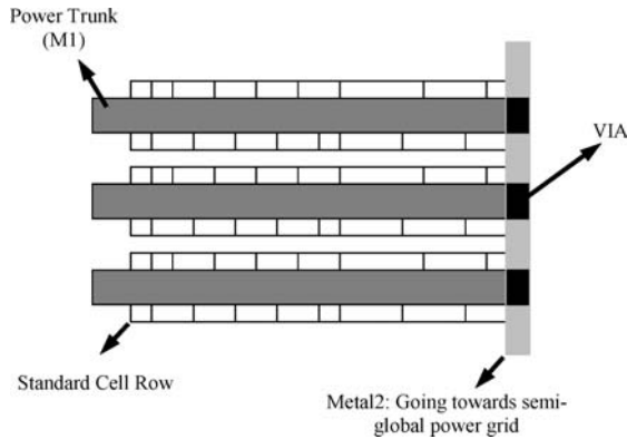
Fig. 2. A local power distribution network for a typical standard cell design consisting of power trunks in a comb-like structure connecting to the semi-global power grid through metal2.
