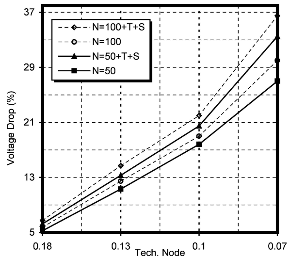
Fig. 8. Total worst-case voltage-drop increase as a function of technology node in the presence of maximum interconnect temperature ( T ) and surface scattering/barrier effects ( S ), while allocating 10% of the routing area to the power network and 5% of the substrate area for decoupling capacitors.
