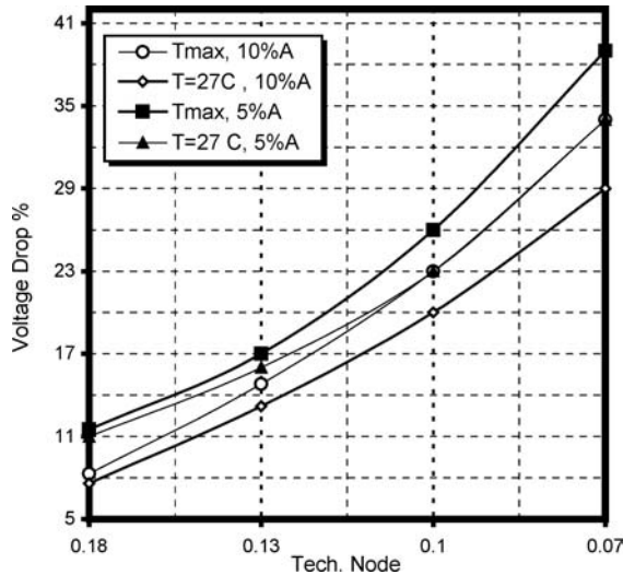
Fig. 4. Worst-case percentage of voltage drop increase as a function of technology node for combined global/semi-global power grids considering the effects of self-heating, while allocating 5% and 10% of the routing area to the power distribution network, respectively.
