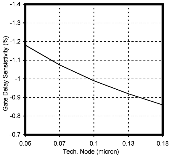
Fig. 10. Sensitivity of the cell delay ( SDV_{dd} ) to the fluctuations of the supply voltage V_{dd} for different technology nodes. Y-axis values show the percentage increase in cell delay for each percent decrease in V_{dd} at the specific technology node.
