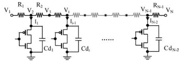
Fig. 3. Magnified view of a trunk segment, containing the resistive network of local power supply network to a series of inverters connected to the intermediate nodes and the decoupling capacitances C_d 's.
