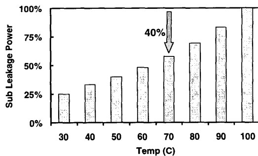
Figure 10: Subthreshold leakage power reduces with lower temperature.
