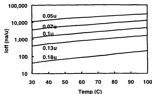
Figure 3: Estimated subthreshold leakage currents of deep submicron transistors
