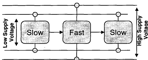
Figure 2: Logic with multiple supply voltages
