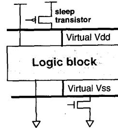
Figure 7: Supply gating or Sleep Transistor technique
