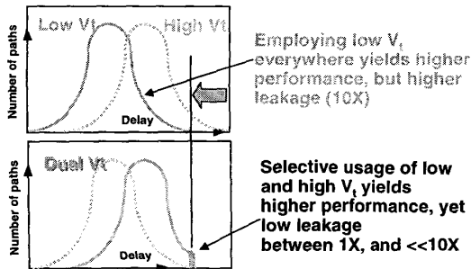
Figure 5: Dual V_t design methodology
