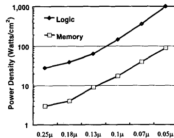
Figure 8: Comparing logic and memory power density
