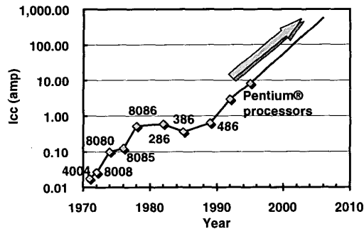
Figure 9: Power supply currents will grow tremendously
