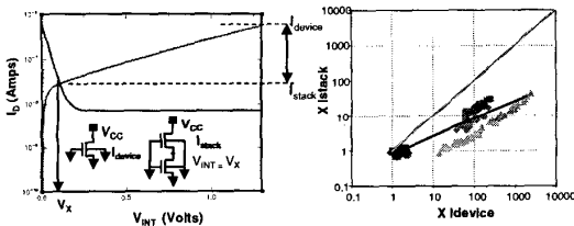
Figure 6: Stack effect to reduce subthreshold leakage
