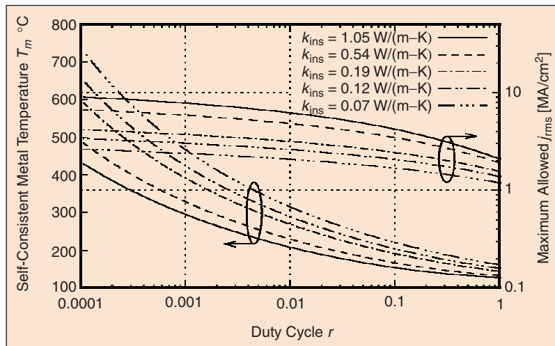
9. Self-consistent solutions for maximum allowed j_{\text{rms}} and T_m for metal 6 in a 180-nm technology for a symmetric bipolar waveform for R = 0.5 for different dielectrics.
