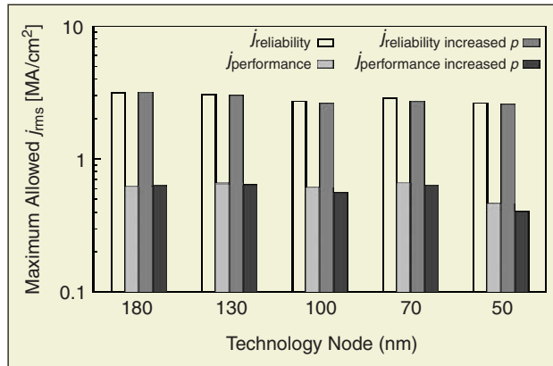
15. Comparison of j_{\text{rms}} values obtained from reliability and electrical performance considerations for top-layer metal for various ITRS technology nodes with and without taking into account increased resistivity due to surface scattering and barrier materials.
