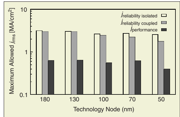
16. Maximum allowed j_{\text{rms}} for top-layer metal of ITRS technologies for symmetric bipolar currents with and without thermal coupling from neighboring lines. Also shown is the j_{\text{rms}} from performance considerations.
