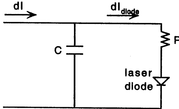
Figure 5.4. Equivalent circuit diagram for laser.
