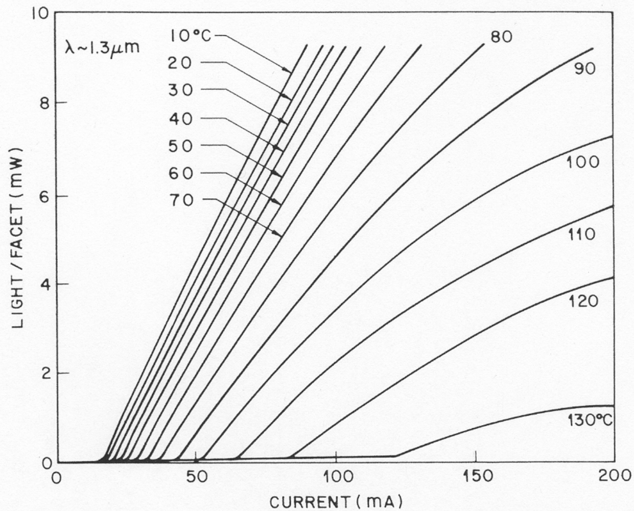
Fig. 5.25 L-I characteristics of a 1.3-μm InGaAsP DCPBH laser at different temperatures.
