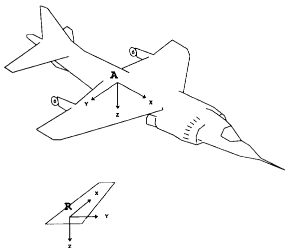
FIG. 1. Aircraft coordinate systems (R—runway, A—aircraft).
