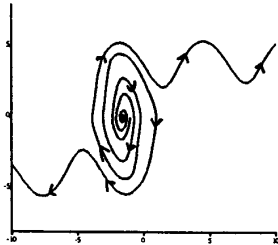
Figure 5: Response of the Zero Dynamics (Initial Condition q_1(0) = -1.35 ) and a Portion of the Phase Portrait
