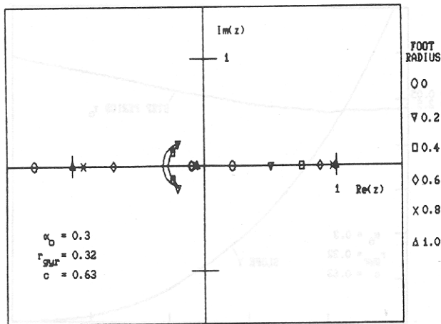
Fig. 9. Locus of the three step-to-step eigenvalues for the walking cycles plotted in Fig. 8, with foot radius as the parameter. In this example one eigenvalue (for the "totter mode") lies outside
