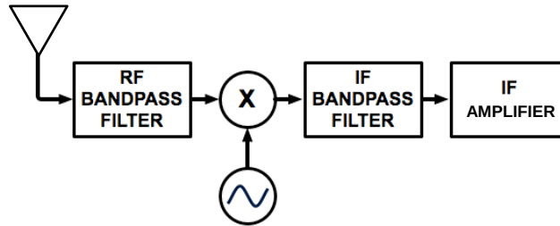
Superheterodyne Basic Receiver
