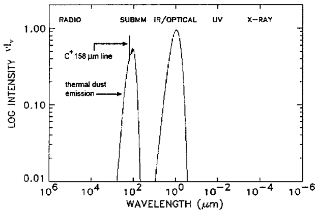
Fig. 4. Spectrum of our Milky Way galaxy showing that at least one-half of the luminous power is emitted at submillimeter wavelengths. The intensity of the ionized carbon emission line at 1.9 THz shows how incredibly abundant this element is (the most after hydrogen, helium, and oxygen) (courtesy of D. Leisawitz et al. [10] and W. Langer, Herschel Space Observatory archive, JPL).
