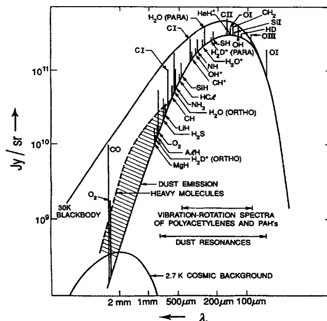
Fig. 2. Radiated energy versus wavelength showing 30-K blackbody, typical interstellar dust, and key molecular line emissions in the submillimeter (reprinted from [9]).
