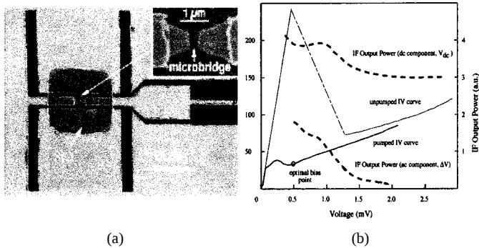
Fig. 16. (a) 2.5-THz niobium HEB twin-slot antenna mixer. (b) Current-voltage characteristics with and without LO power applied. Also shown is the dc ( V_{dc} ) and ac ( \Delta V ) components of the IF output power (courtesy of [115] and [116]).
