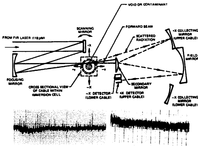
Fig. 9. 2.5-THz cable void inspection system and plots of scattered power from: (a) void-filled and (b) solid cable. Peaks are indicative of void size (courtesy of [49]).
