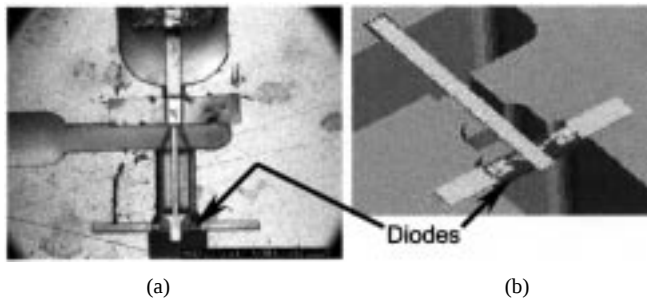
Fig. 18. Terahertz Schottky diode multiplier chips fabricated monolithically from GaAs. (a) 800-GHz balanced doubler with thin membrane frame mounted in waveguide block [171]. (b) 2400-GHz waveguide-mounted substrateless-doubler schematic (currently in process at the JPL) [167].
