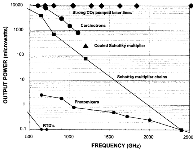
Fig. 19. Performance of some CW sources in the submillimeter-wave range. Data: Schottky varactor (JPL recent results), RTD [155], [156], Photomixer [52], [146], Carcinotron [Online]. Available: http://www.pi1.physik.uni-stuttgart.de/indexjs.html , Laser lines [185].
