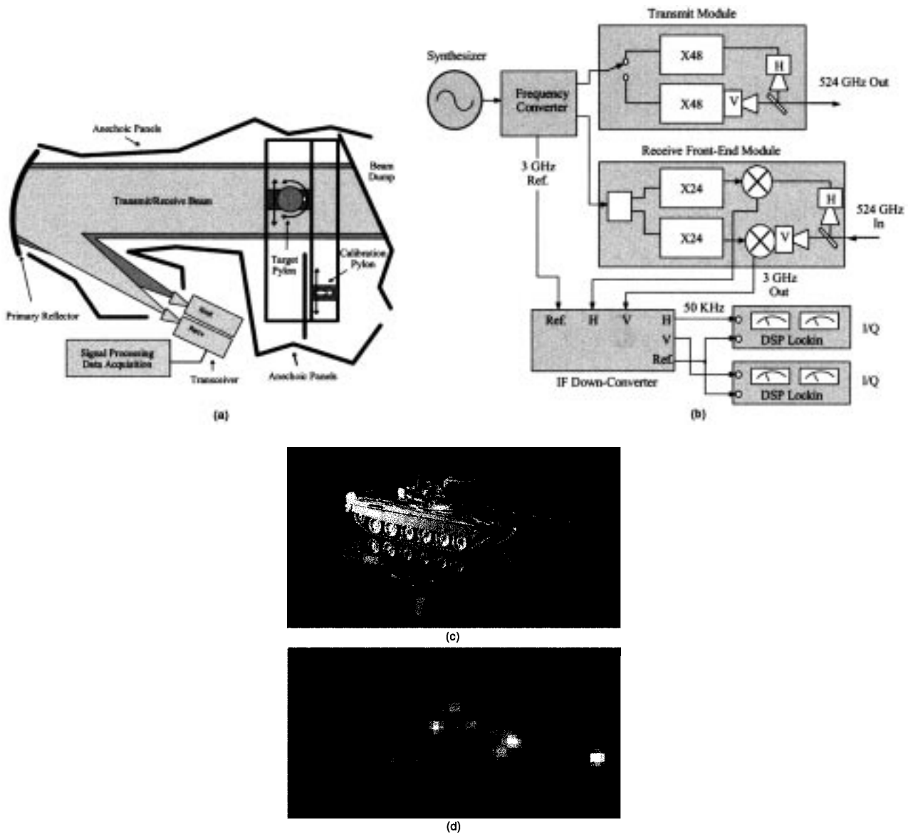
Fig. 11. Terahertz RCS system. (a) Compact range layout and submillimeter-wave transmit/receive arrangement. (b) Transceiver block diagram. (c) Optical image of scale model tank. (d) Processed submillimeter-wave radar image—cross section of 3-D image (courtesy of [54]).
