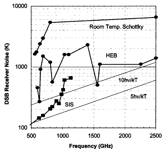
Fig. 15. Heterodyne receiver noise temperatures (SIS, HEB, and Schottky) versus frequency in the submillimeter range. SIS/HEB results can be found in the 11th and 12th International Space Terahertz Technology Conference and represent several receiver development groups and operating conditions (hence, the scatter). Schottky data are recent planar diode results from the University of Virginia, Charlottesville, and the JPL.
