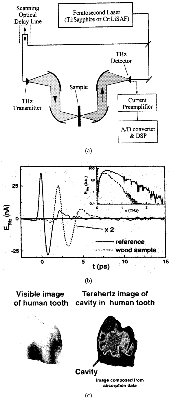
Fig. 12. (a) T-ray imager schematic [58]. (b) Time- and frequency-domain images of terahertz transmission through a piece of wood [55]. (c) 2-D contour plot of terahertz transmission through extracted tooth [56] (courtesy of [55], [56], and [58]).
