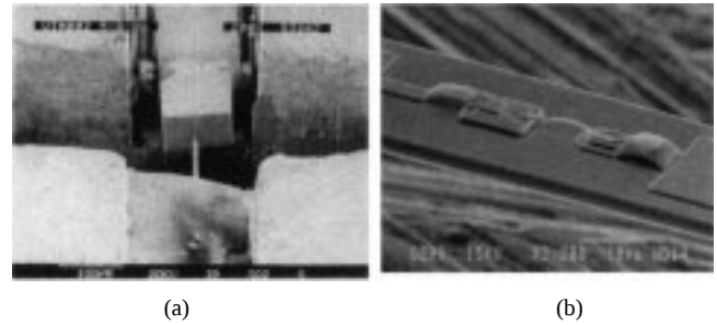
Fig. 13. (a) Whisker-contacted Schottky honeycomb diode circa 1980 for 200-GHz operation in waveguide downconverter. Chip width is 125 \mu\text{m} . (b) Planar integrated submicrometer area Schottky diode on 3- \mu\text{m} -thick \times 30- \mu\text{m} -wide GaAs membrane for operation at 2500 GHz, also coupled to a waveguide mount.
