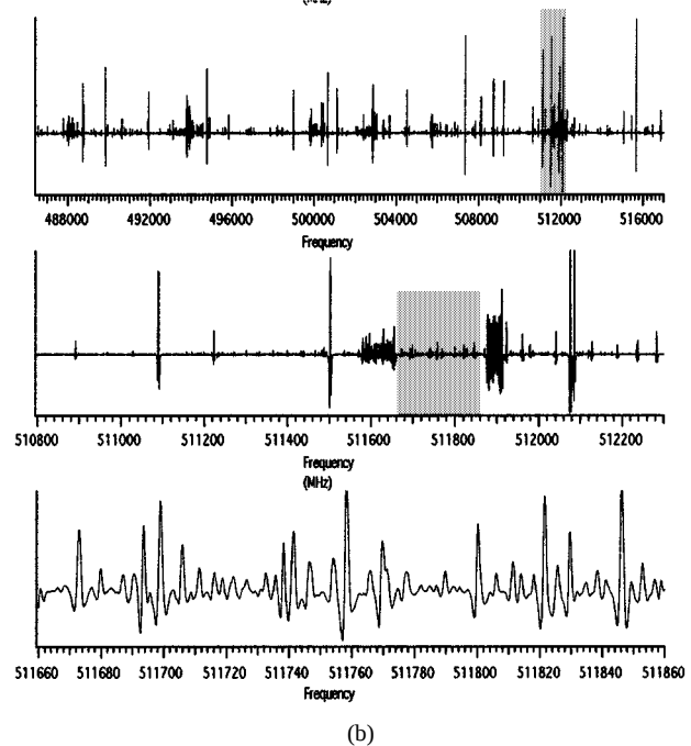
Fig. 7. (a) FASST schematic. (b) Spectral plots at 500 GHz in increasing frequency resolution sweeps (top to bottom) for a combination of pyrrole, pyridine, and sulfur dioxide at 10 mTorr each (courtesy of [43]).
