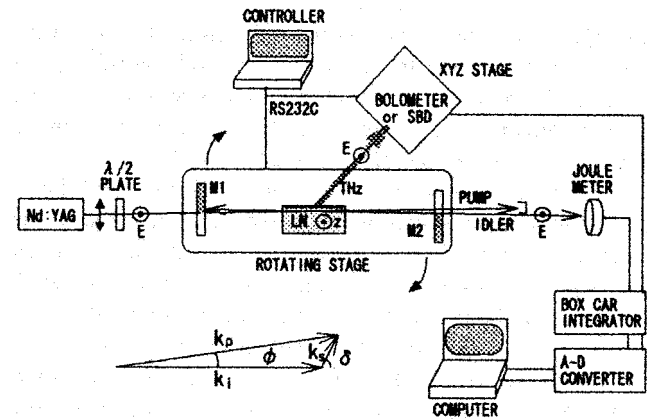
Fig. 20. Terahertz generator based on laser illumination of a lithium–niobate crystal (courtesy of [196], American Institute of Physics).
