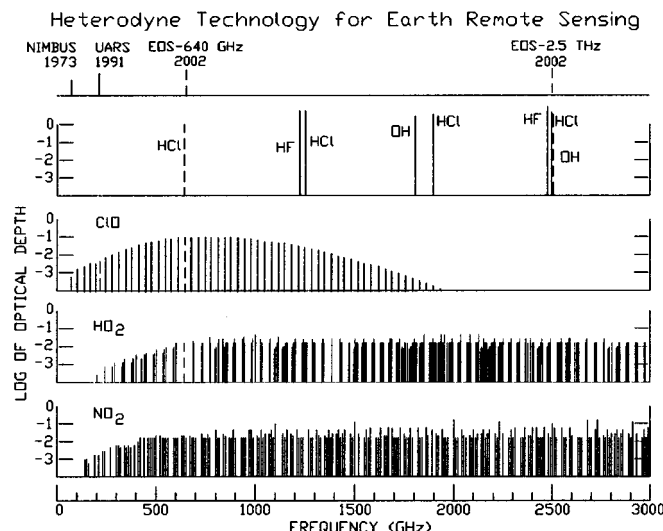
Fig. 5. Spectra of some important molecules in the Earth's upper atmosphere and measurements being addressed by NASA heterodyne instruments. The peak power or minimum frequency for many emission lines occurs in the terahertz region. Figure based on J. Waters, EOS Atmospheres presentation [17].
