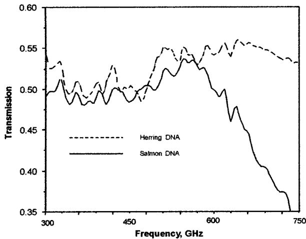
Fig. 8. Comparison of Herring and Salmon DNA transmission spectra using an FTS system (courtesy of [46]).
