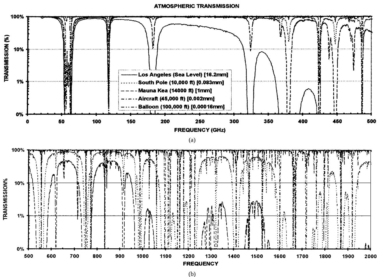
Fig. 1. Atmospheric transmission in the terahertz region at various locations and altitudes for given precipitable water vapor pressure (in millimeters). (a) 0–500 GHz. (b) 500–2000 GHz. Data from Erich Grossman using his “Airhead Software” [6].
