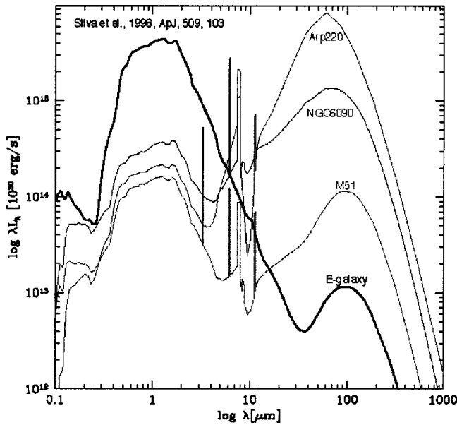
Fig. 3. Energy output versus wavelength for galaxies of ascending ages (E-galaxy = youngest, Arp220 = oldest) showing the advantages of terahertz detection systems for probing the early universe [courtesy of W. Langer, Herschel Space Observatory archive, Jet Propulsion Laboratory (JPL)].
