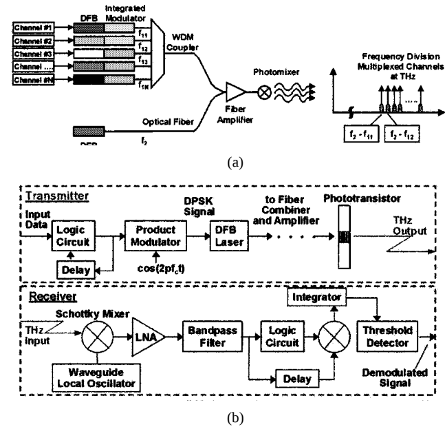
Fig. 10. (a) Optically diphexed terahertz transmitter source based on 1.5- \mu m fiber technology and terahertz power generation through photomixing. (b) Gigabit data-rate transmit/receive module based on this technology (courtesy of [52]).
