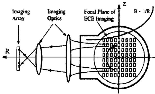
Fig. 6. Diagram of 2-D plasma ECE heterodyne imager using linear array of receive antennas for \sim 100 GHz. LO power is incident from the rear of the array and distributed to each element by a cylindrical mirror (courtesy of [36], American Institute of Physics).
