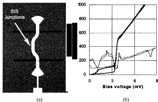
Fig. 14. (a) 1200-GHz SIS tunnel junctions integrated on planar slot antenna circuit. (b) Current-voltage relationship and IF output signal for 77- and 300-K blackbody loads. Equivalent input receiver noise temperature is 650-K DSB at 1130 GHz (courtesy of A. Karpov [100]).
